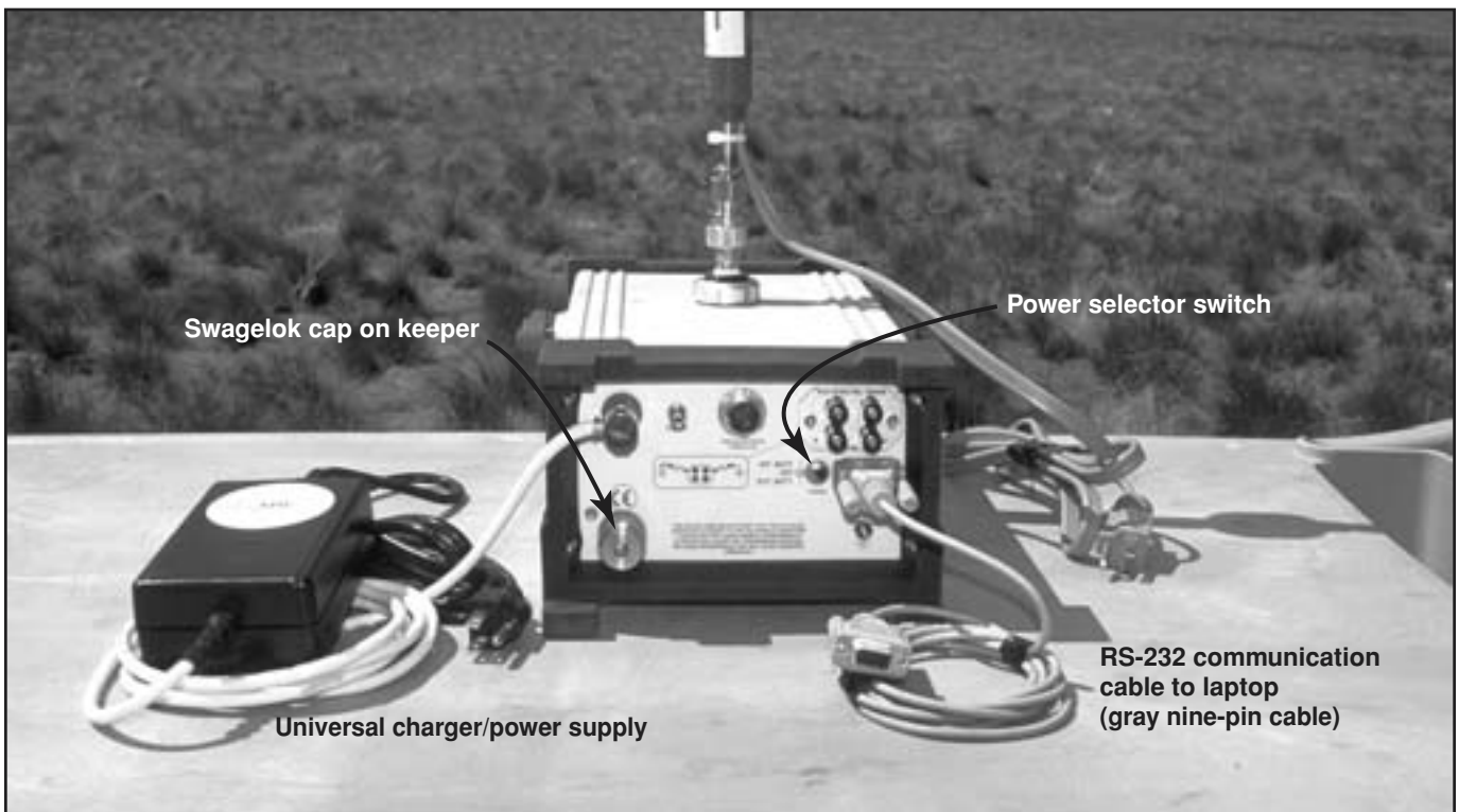
Figure 3—Back-panel view of the DataRAM4.
