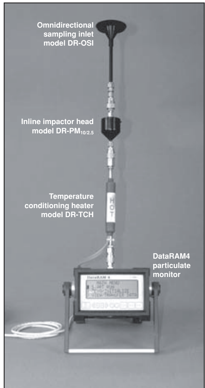
Figure 2—The DataRAM with all three ambient monitoring accessories.
